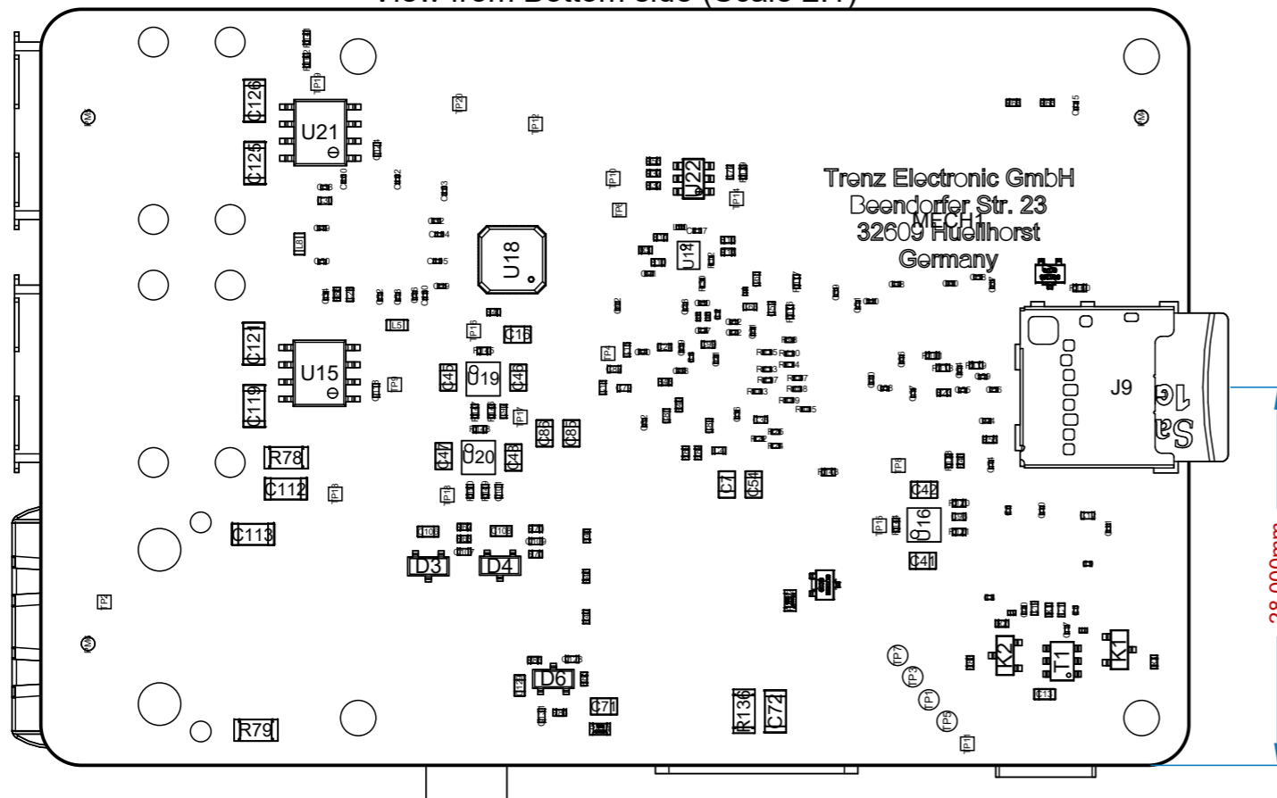
View from Bottom side (Scale 2:1)
