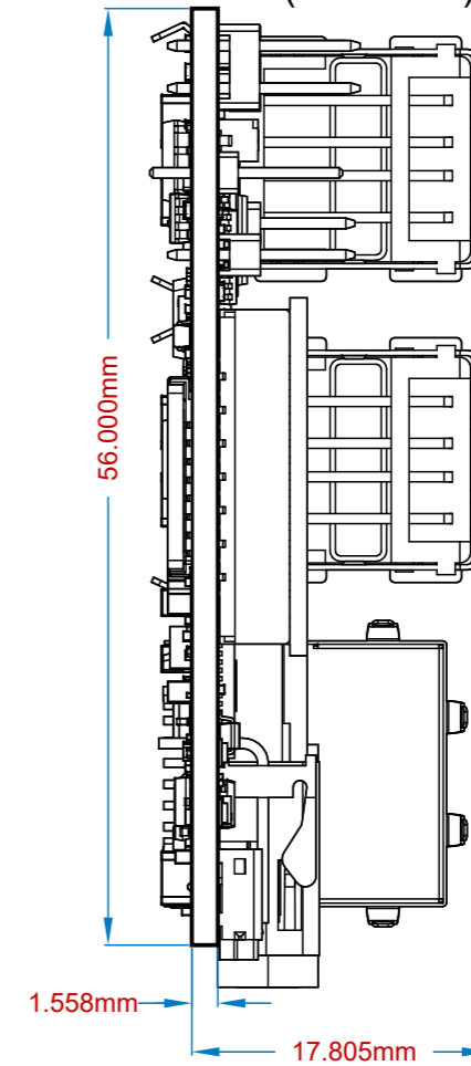
View from Left side (Scale 2:1)
